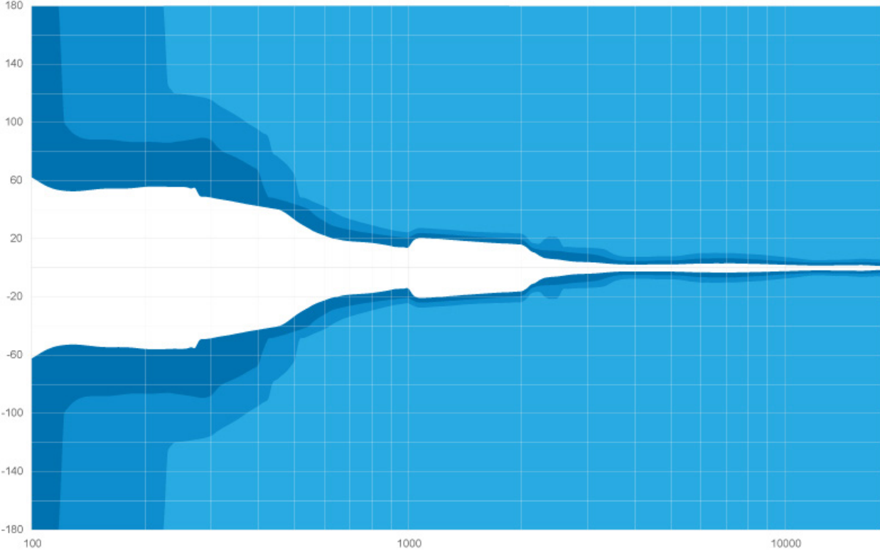
ARES 12 Vertical beamwidth
