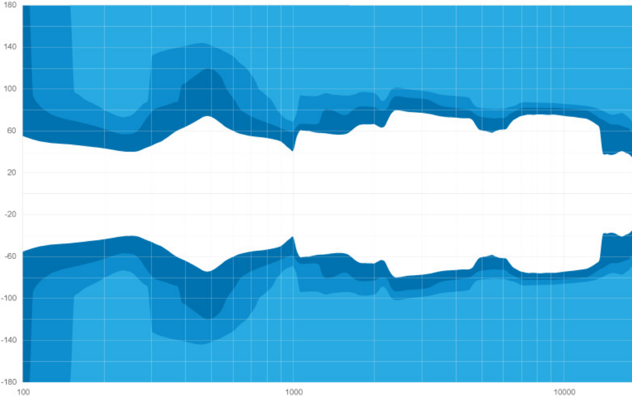
ARES 12 Horizontal beamwidth
